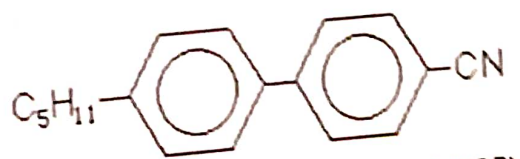
5CB p - n pentyl- p '-cyanobiphenyl (PCB)
